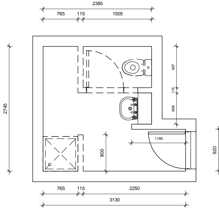
Demolished Layout 1:50
