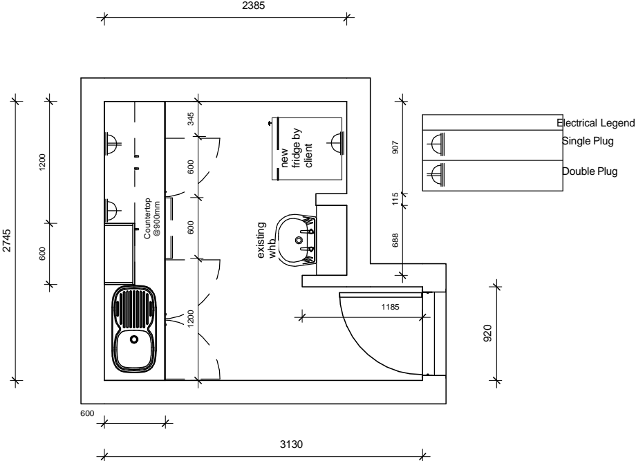
Proposed New Kitchen Layout
