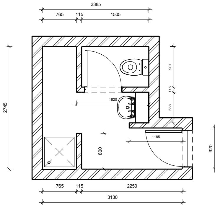
Existing Change Room 1:50
