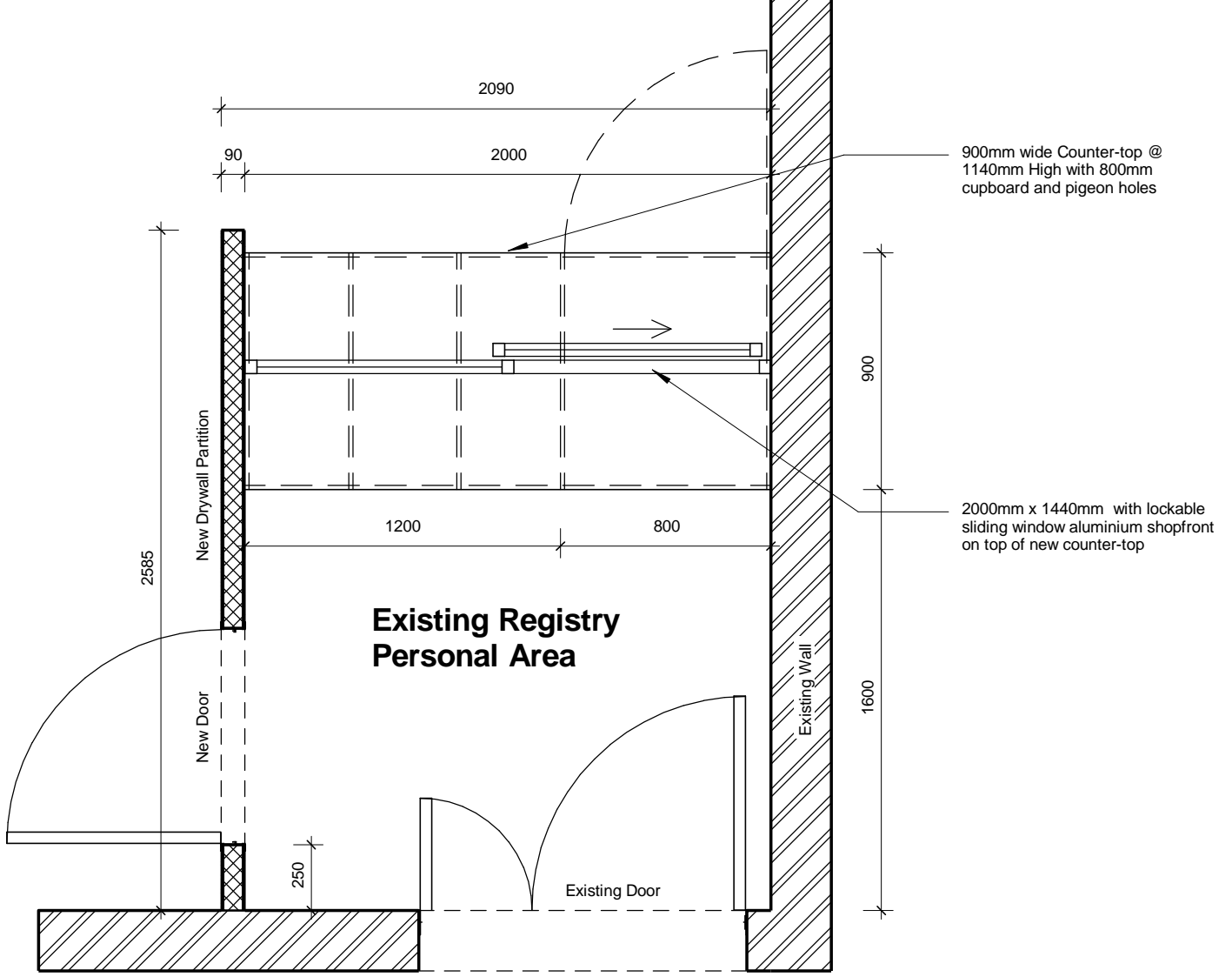
Drawing No: 001 Registry Personal - Plan 1:25
