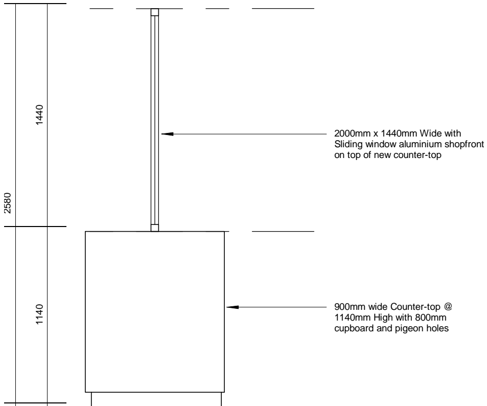
Drawing No: 001 Registry Personal - Typical Section 1:25
