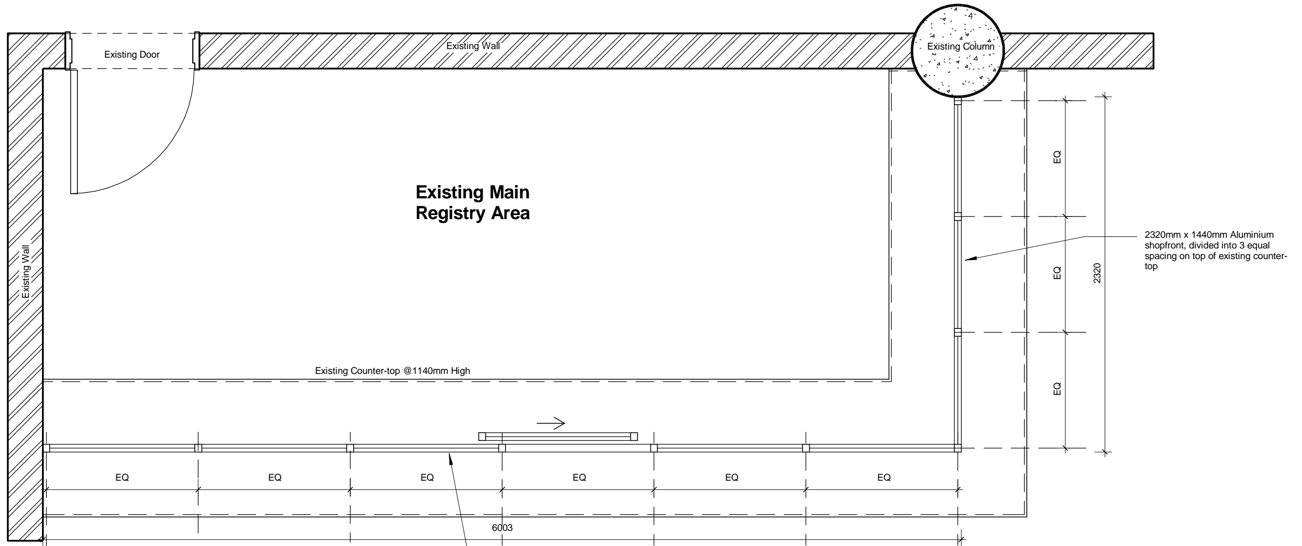
Drawing No: 002 Main Registry - Plan 1:25
