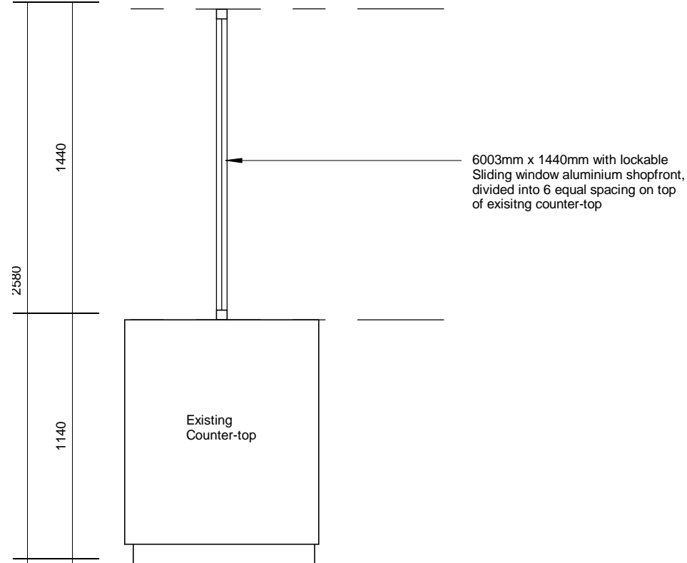
Drawing No: 002 Main Registry - Typical Section 1:25
