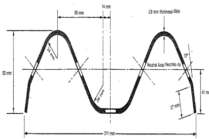
PROFILE DIMENSIONS/PROFIEL AFMETINGS
