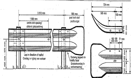
SPLICES & POST BOLTS/SPLIT-EN PAALBOUTE
