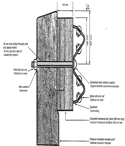
INSTALLATION/INSTALLERING
