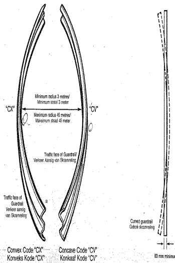
TYPICAL GUARDRAIL/TIPIESE SKRAMRELING
