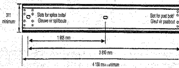
TYPICAL GUARDRAIL/TIPIESE SKRAMRELING
