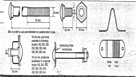
SPLICES & POST BOLTS/SPLIT-EN PAALBOUTE
